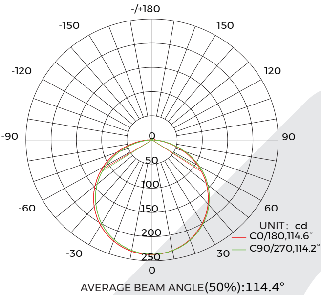
Light distribution
